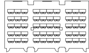
CLASSROOM 104 PPL
